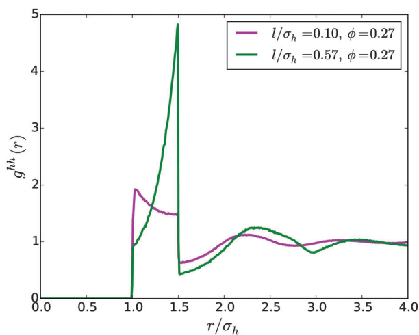
Fig. 6 Bulk head-head radial distribution functions g^{hh}(r) of the coexisting MMSW liquid at packing fraction \phi = 0.27 for bond length l/\sigma_h = 0.1 (magenta curve) and l/\sigma_h = 0.57 (green curve), as function of the distance r . The repulsive beads increase on average the spacing between the attractive beads.
