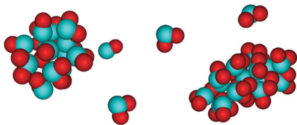
Fig. 9 Disordered clusters of MMSW particles for bond length l/\sigma_h = 0.57 , interaction range \lambda = 1.40 and temperature k_B T/\epsilon = 0.31 . (Left) N = 15 , \phi = 0.011 , (right) N = 20 , \phi = 0.015 .
